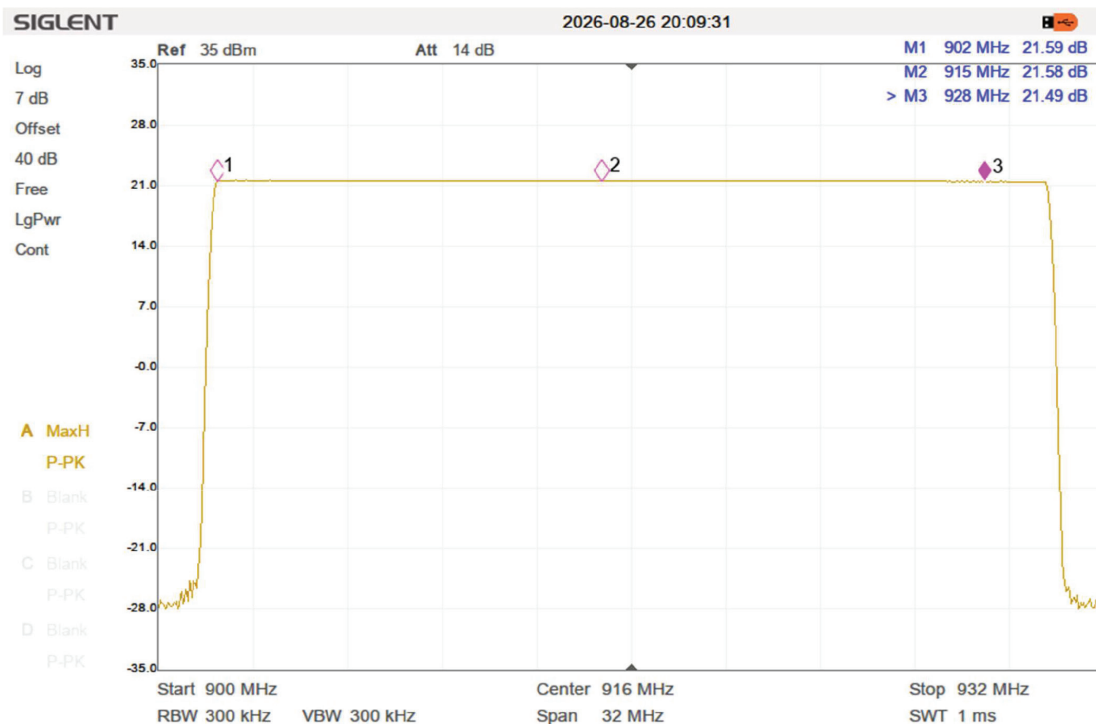
Figure 2. PA output power. Input RF signal CW 8dBm
