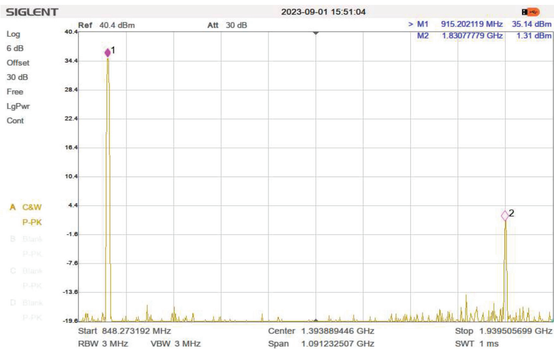
Figure 6. 2nd Harmonic. Output Power CW 35 dBm
