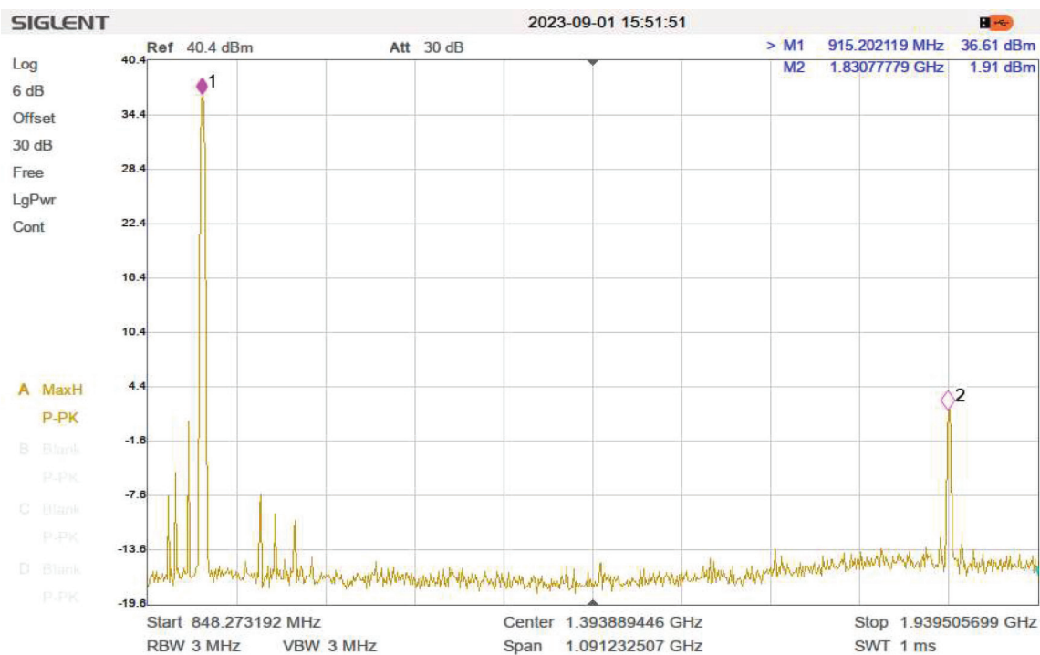
Figure 5. 2nd Harmonic. Output Power Pulse 36 dBm
